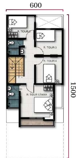
Denah Lantai 2
