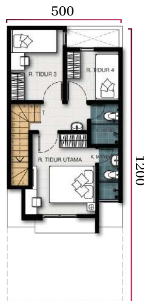
Denah Lantai 2
