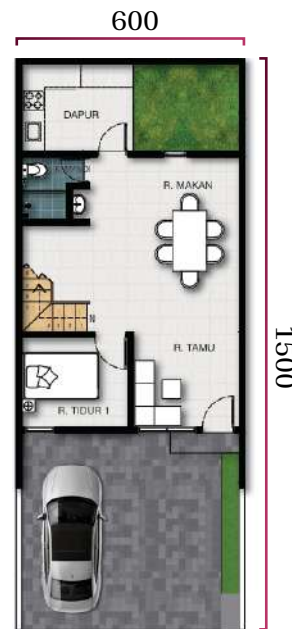
Denah Lantai 1
