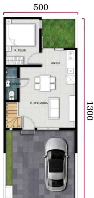
Denah Lantai 1
