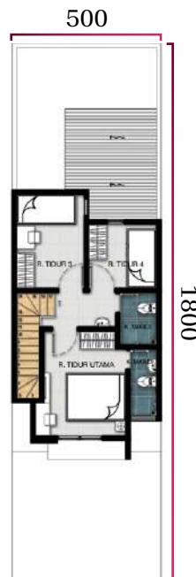
Denah Lantai 2
