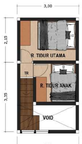
DENAH LT.2 SKALA 1:50
