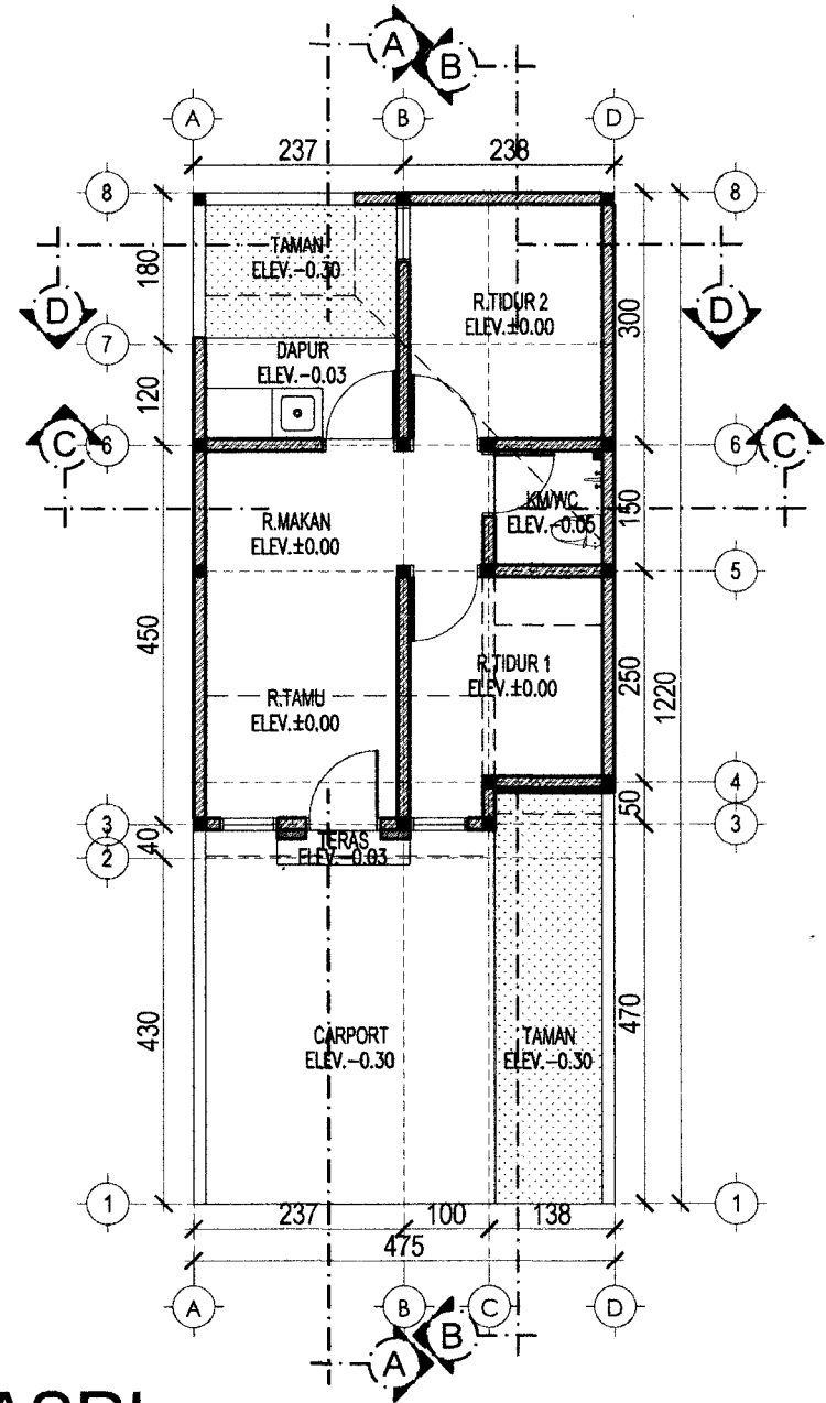
DENAH 31/58 Kav. 4,75 x 12,20 - Skala 1:100
