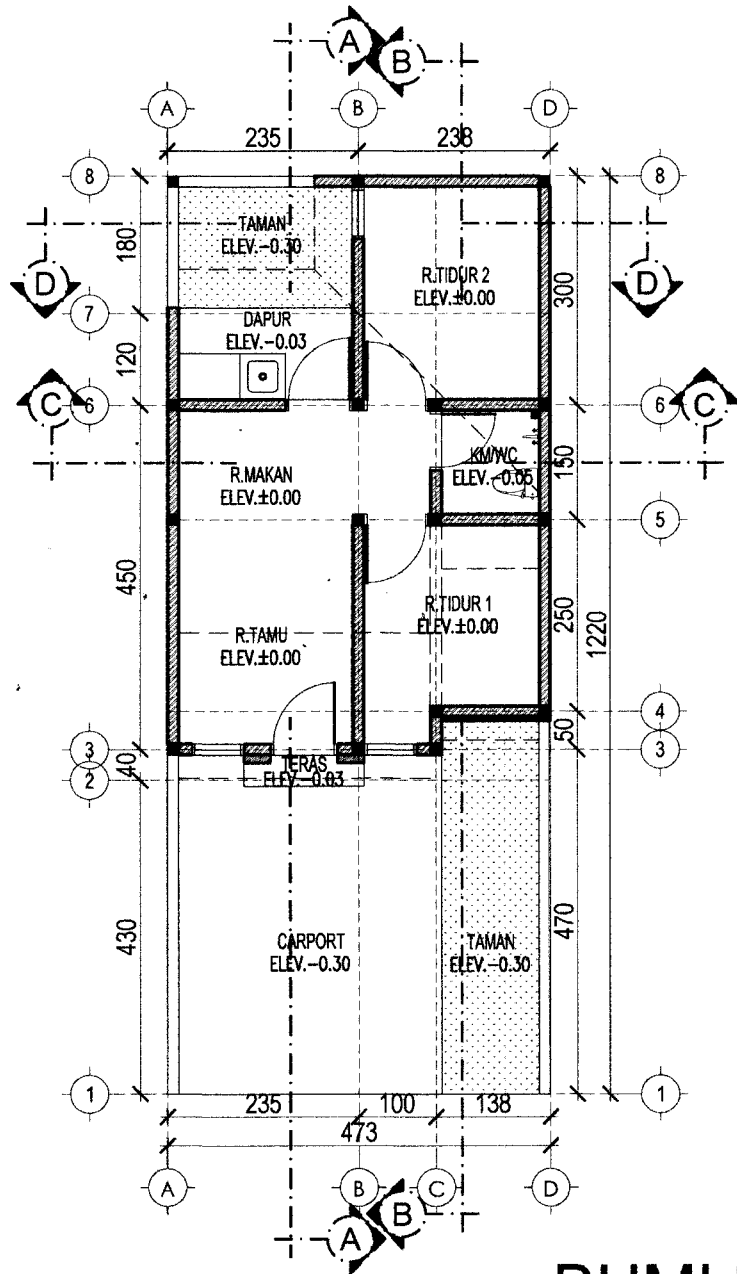
DENAH 31/58 Kav. 4,73 x 12,20 - Skala 1:100
