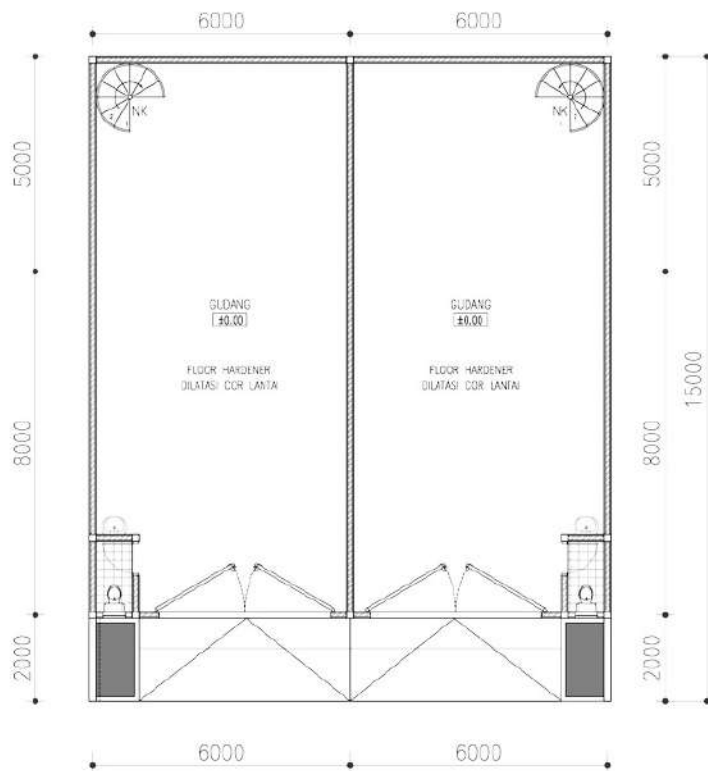
DENAH GUDANG 6x15 SKALA 1:100
