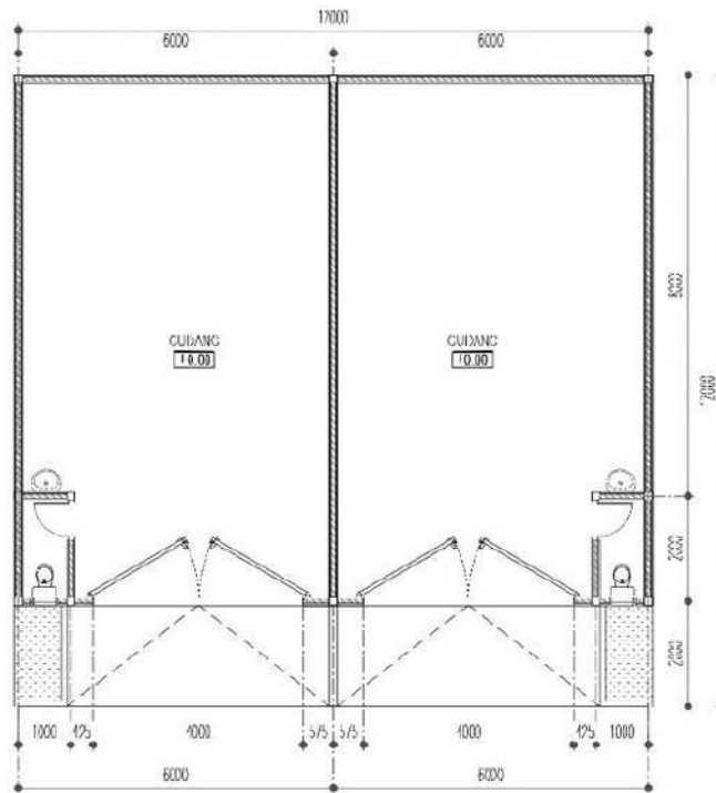
DENAH GUDANG 6x12v SKALA 1:100
