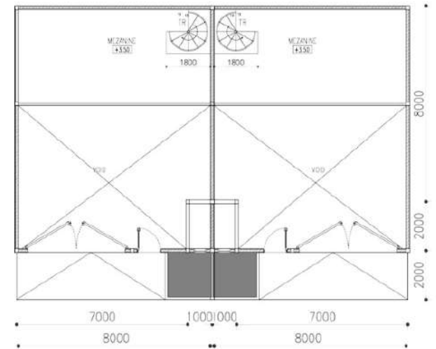
DENAH MEZZANINE SKALA 1:100
