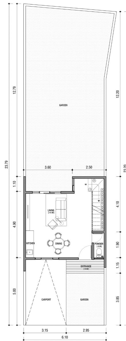
DENAH LANTAI 1 LB : 83 M2
