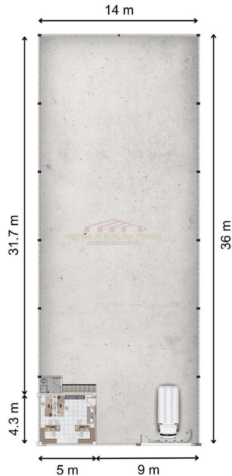
DENAH LANTAI 1
