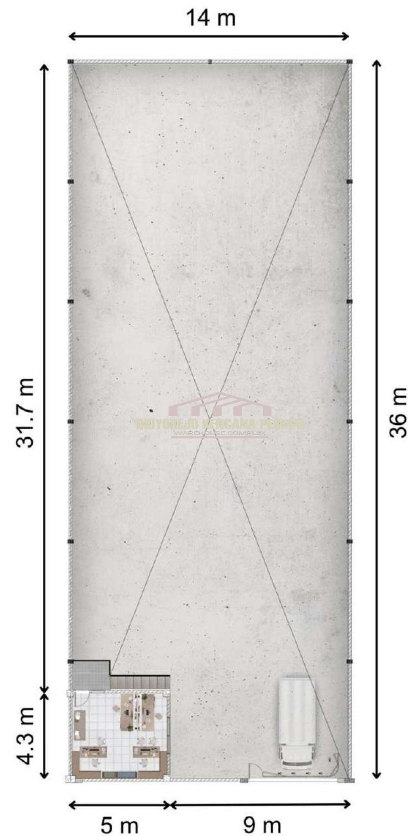
DENAH LANTAI 2
