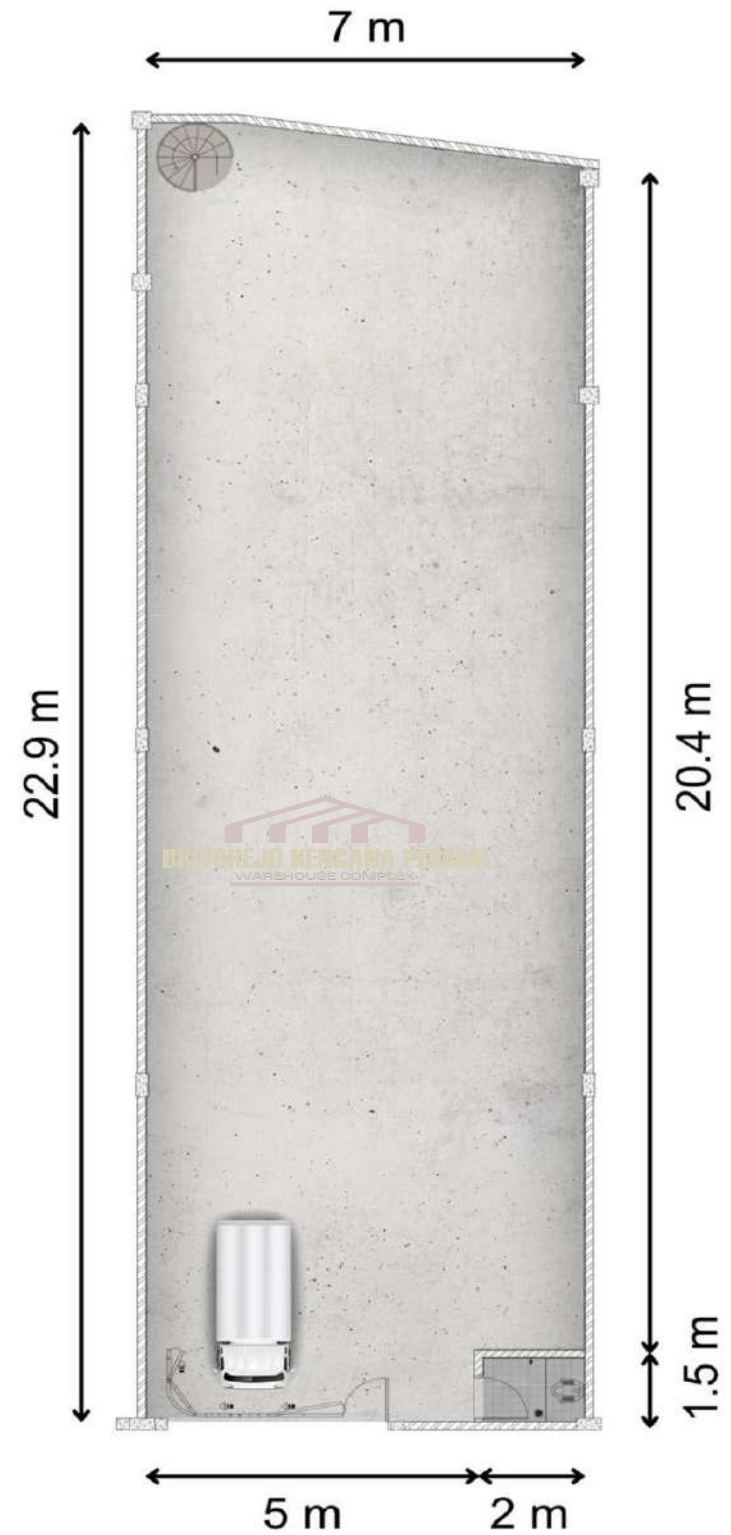
DENAH LANTAI 1
